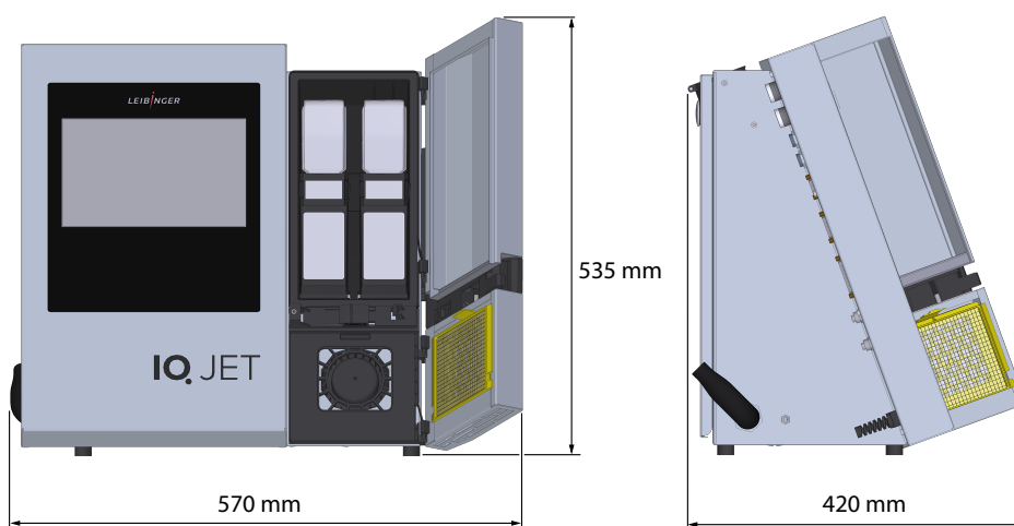
Fig. 2: Dimensions when front doors are open
